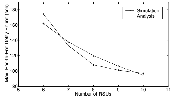
Fig. 4. Maximum end-to-end delay with the number of RSUs.
