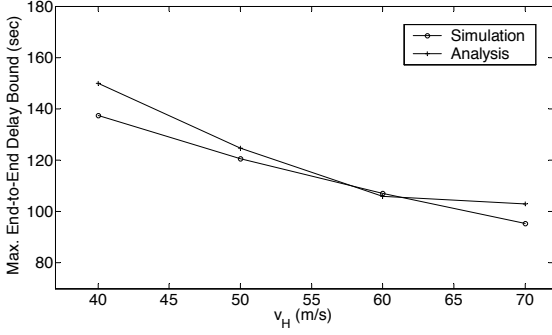
Fig. 10. End-to-end delay bound variation with the vehicle speed difference ( v_H varies, v_L = 30m/s ).
