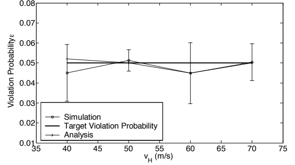
Fig. 11. Delay violation probability variation with the vehicle speed difference ( v_H varies, v_L = 30m/s ).
