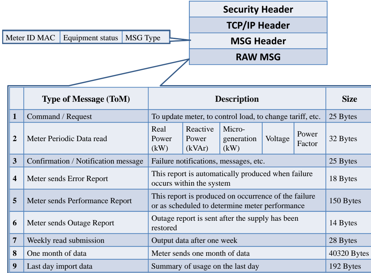
Fig. 2. SG communications packet structure.
