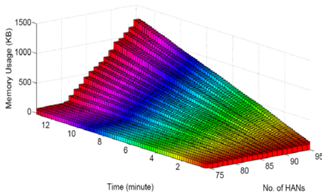
(a) Number of HANs supported by the conventional ECDSA-256 scheme.
